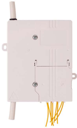
MTeH MINI – Riser Solution – Terminated on Pigtaills
