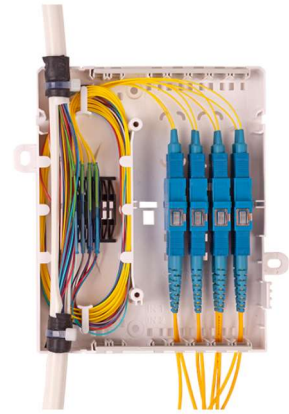
MTeH MINI – Riser Solution – Terminated on Pigtaills
